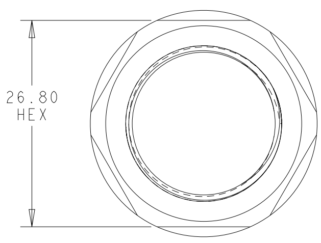
LOCKING NUT DETAIL SCALE 2:1
